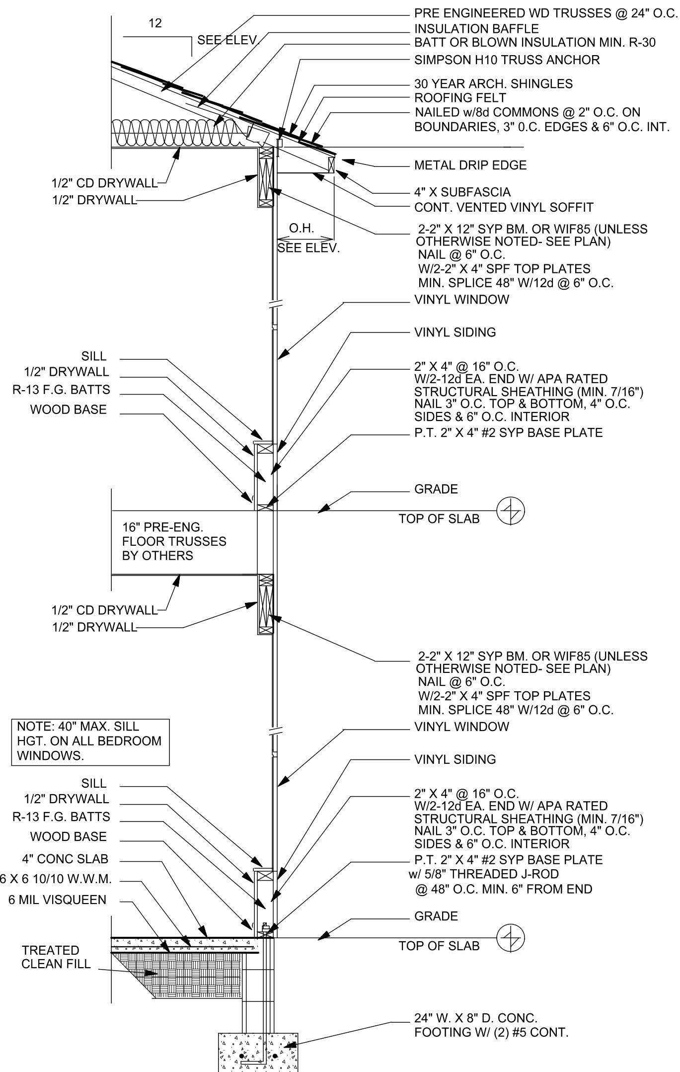
TYPICAL WALL SECTION EXTERIOR FRAME
