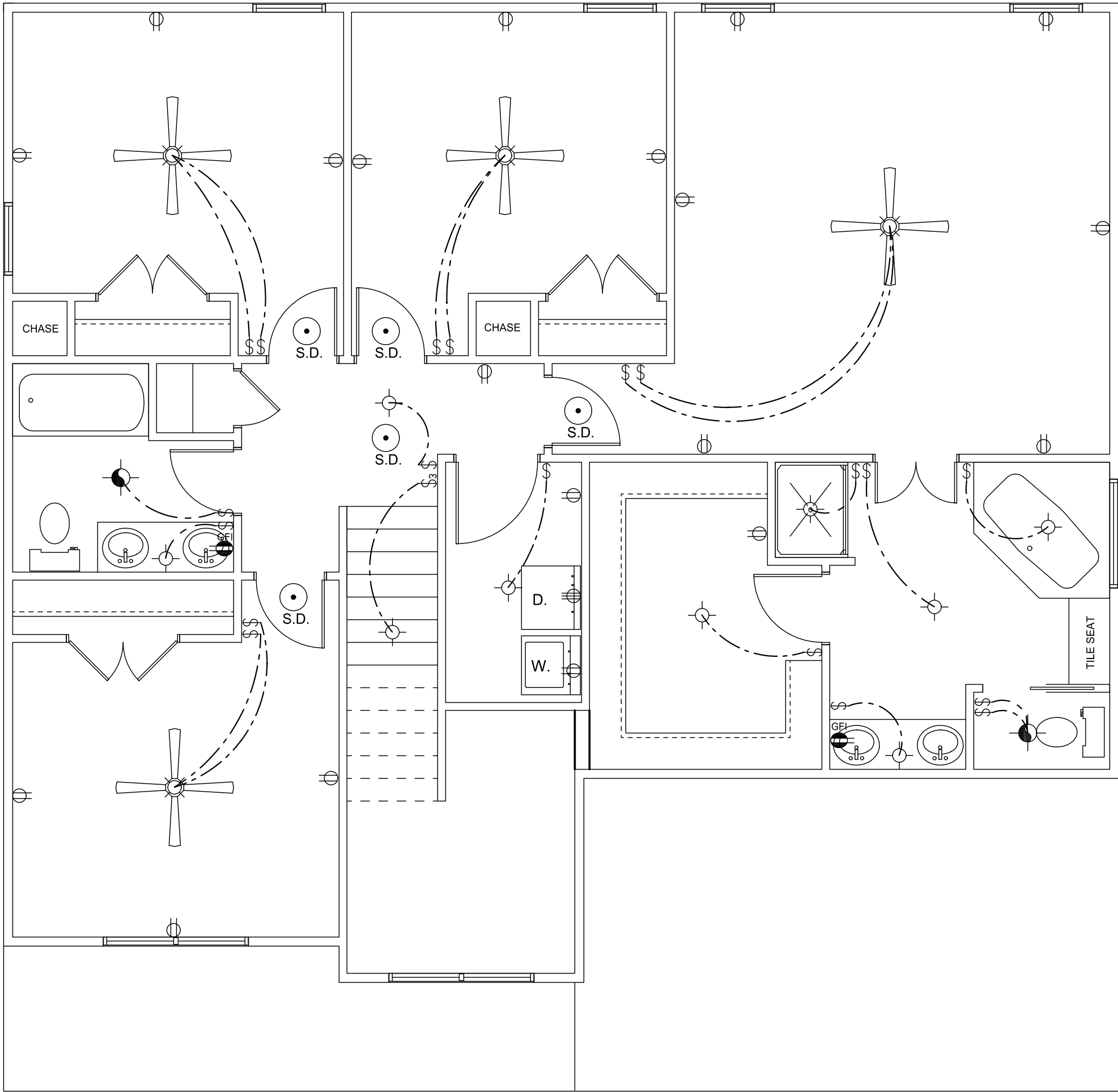
SECOND FLOOR ELECTRICAL PLAN SCALE: 1/4" = 1'-0"
